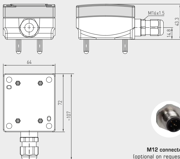
Dimensional drawing
