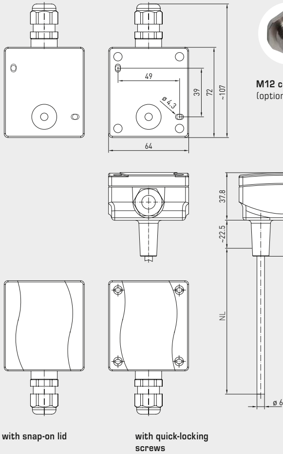
Dimensional drawing
