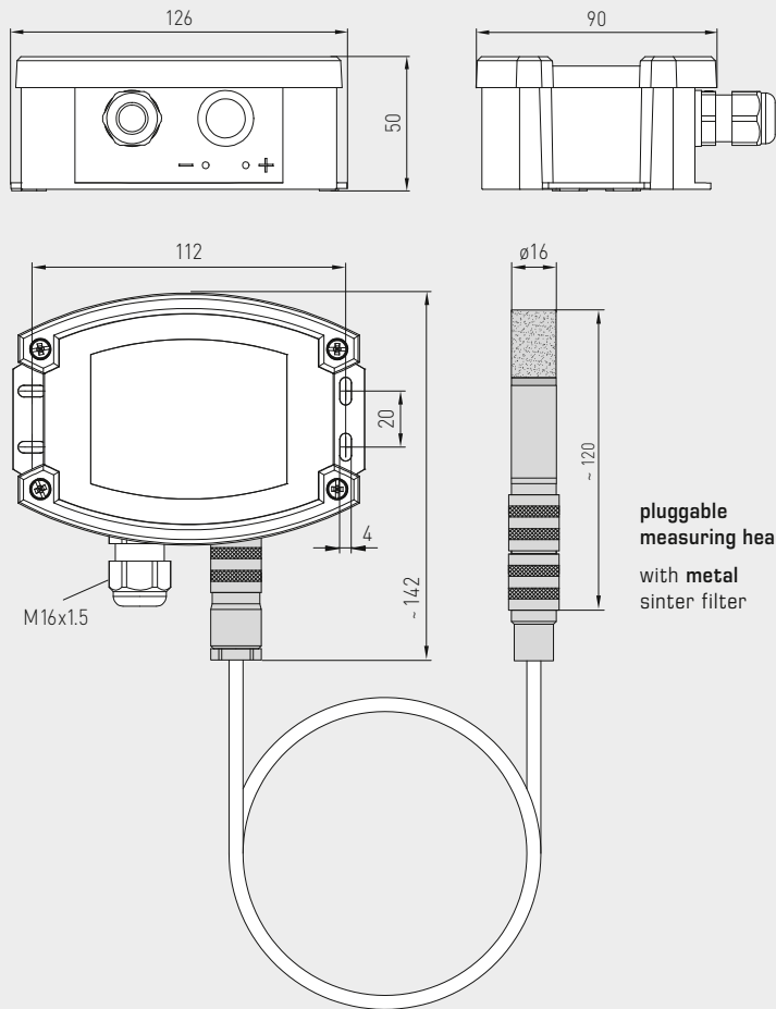
Dimensional drawing
