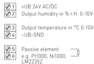
4- or 6-wire connection RFTF-U (passive temperature sensor)
