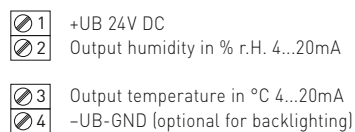
3- or 4-wire connection ** RFTF-I (Transmitter)
