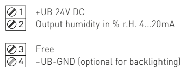
2- or 3-wire connection * RFF-I (Transmitter)
