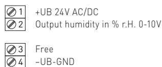
3-wire connection RFF-U
