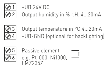
4- or 6-wire connection RFTF-I (passive temperature sensor)
