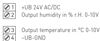
4-wire connection RFTF-U RFTF-U with display
