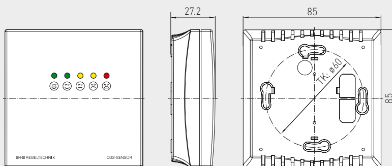
Dimensional drawing (Baldur 1)
