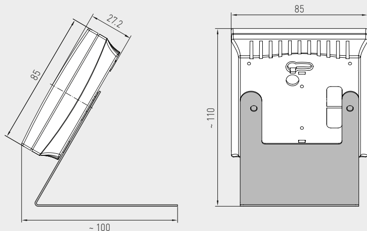
Dimensional drawing with stand holder
