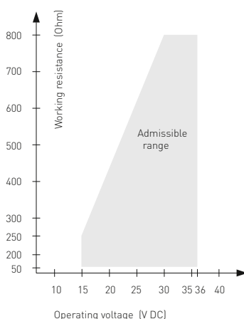
Load resistance diagram
