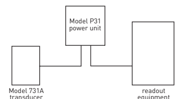
Powering with P31 power unit
