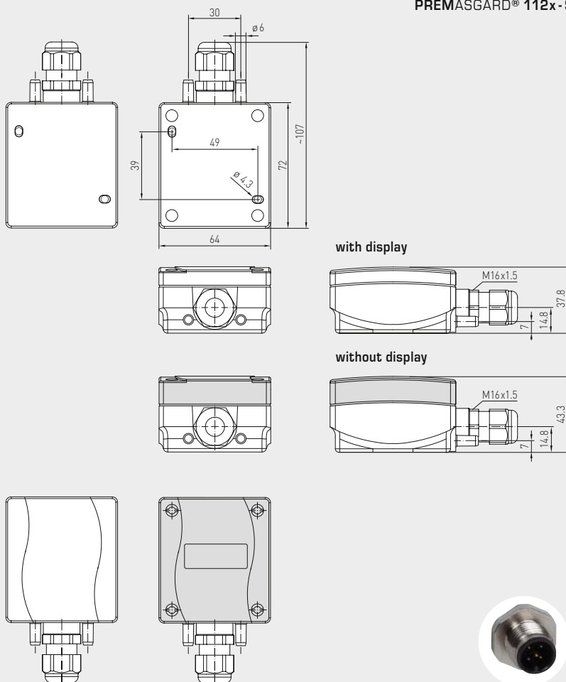
Dimensional drawing
